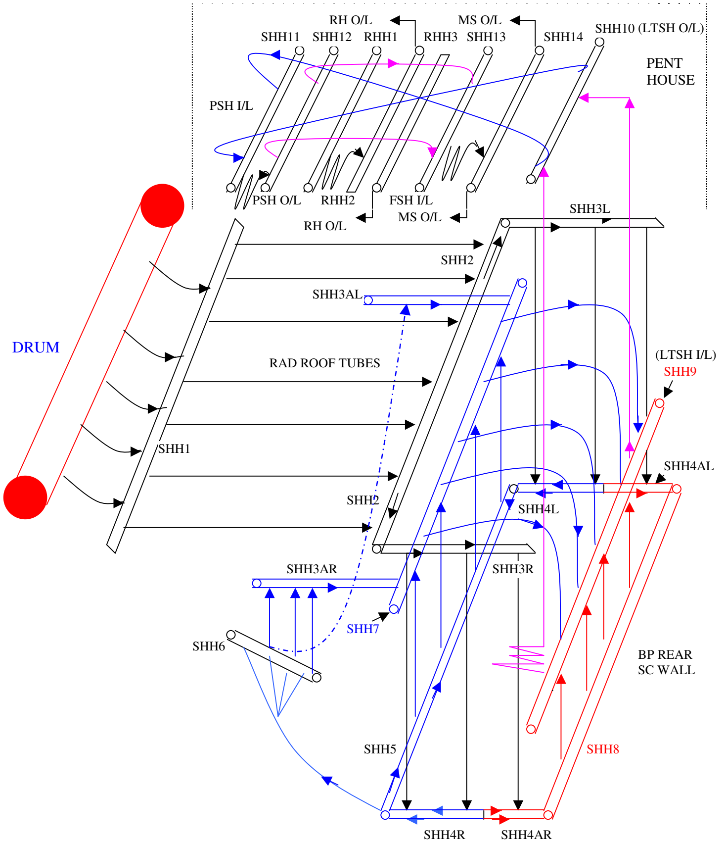
STEAM PATH FROM DRUM OUT LET TO FSH O/L(SHH14)
