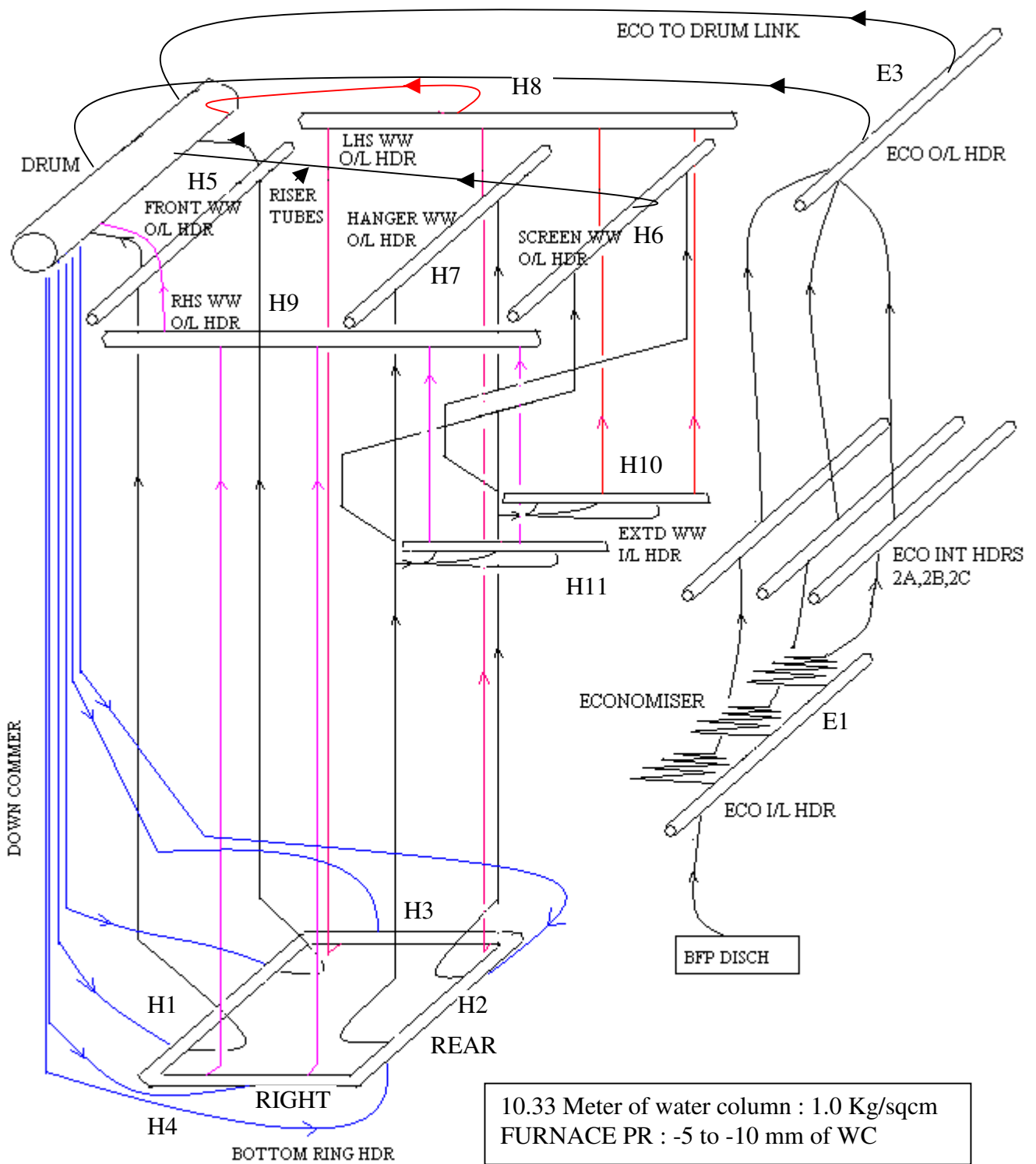
WATER PATH & HEADERS
